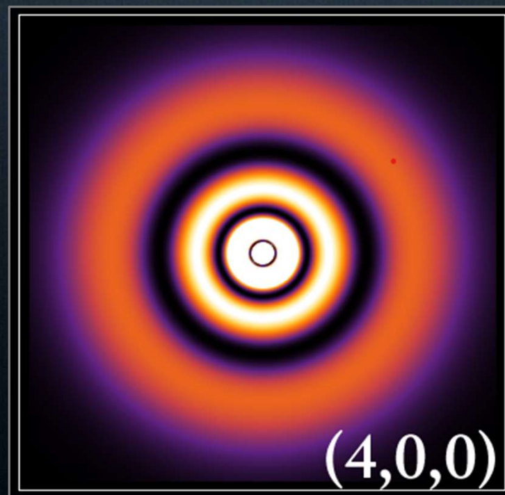
Electron 'Cloud'
