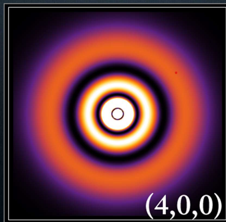
Electron 'Cloud'
