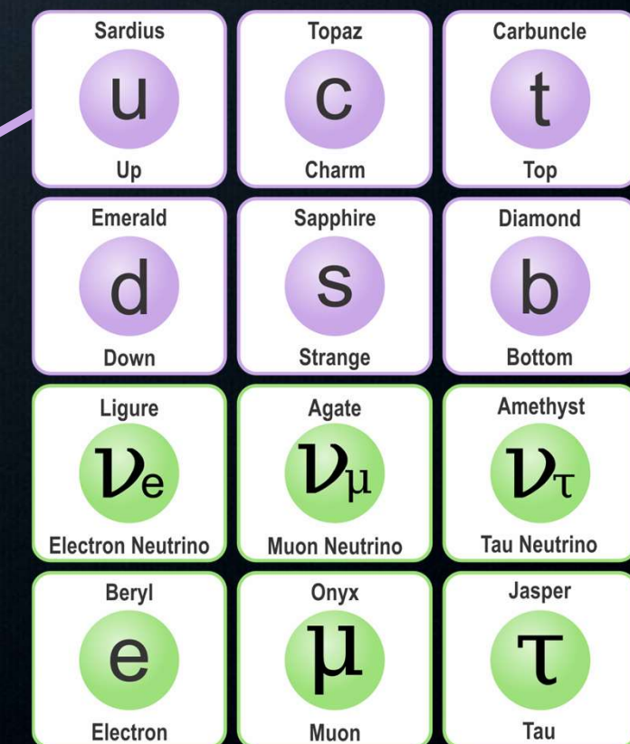
Standard Model
