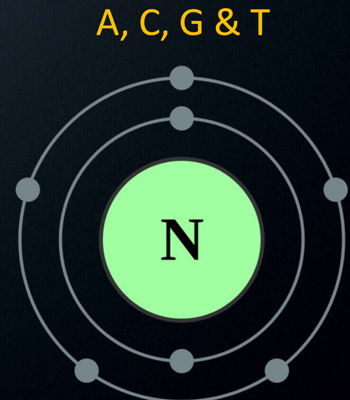
Nitrogenous Bases
