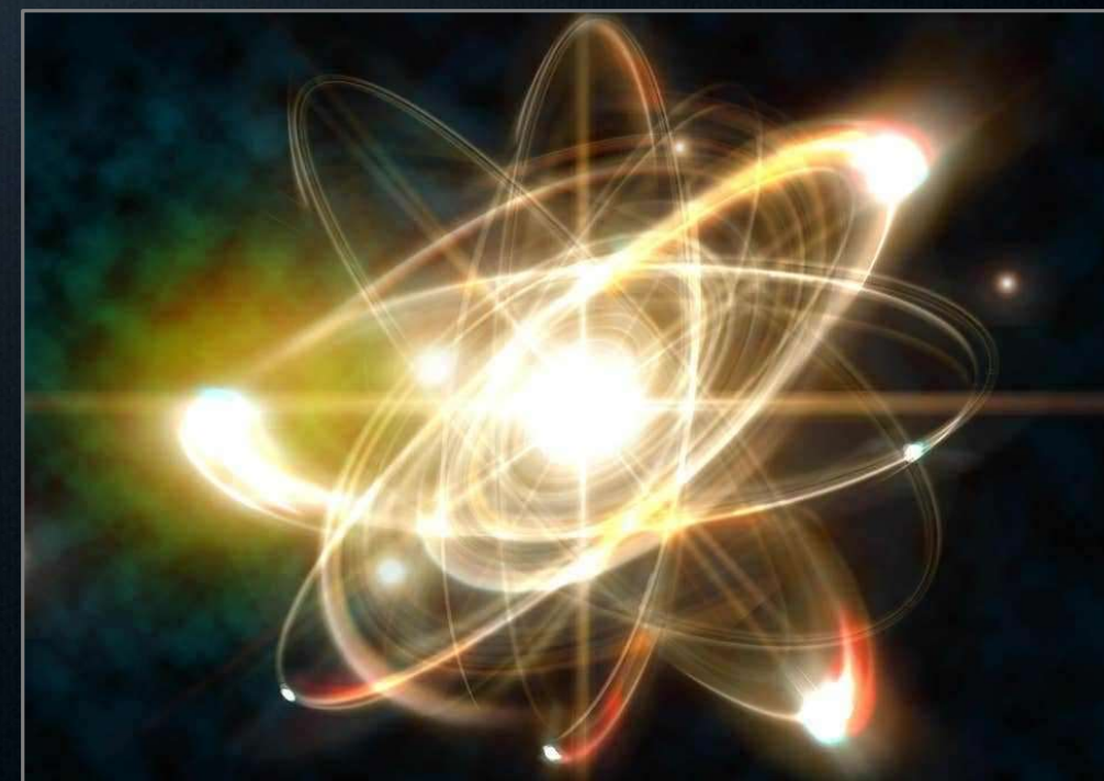
Electron Orbitals
