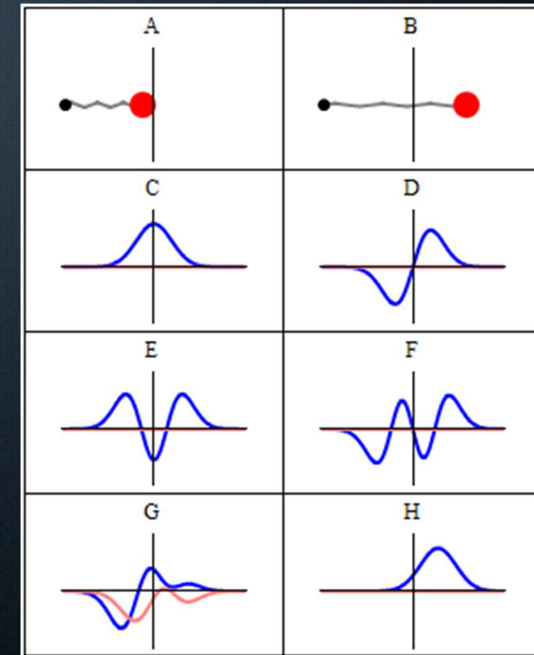
Wave Function
