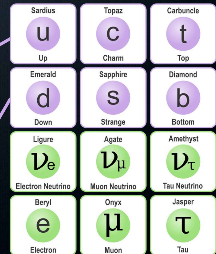
Standard Model
