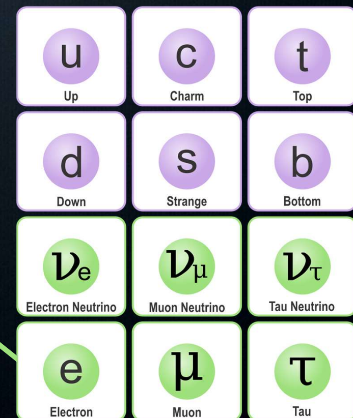
Standard Model
