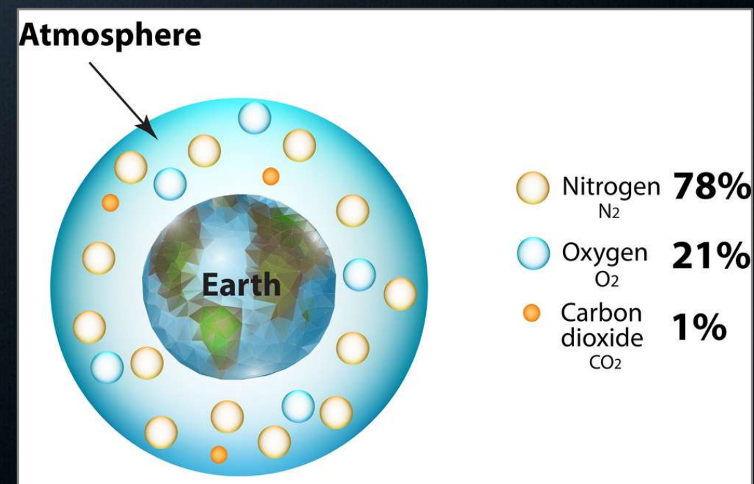
Earth's Atmosphere
