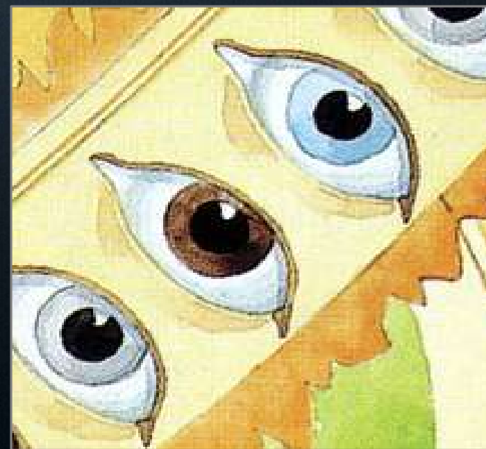
Electrons
