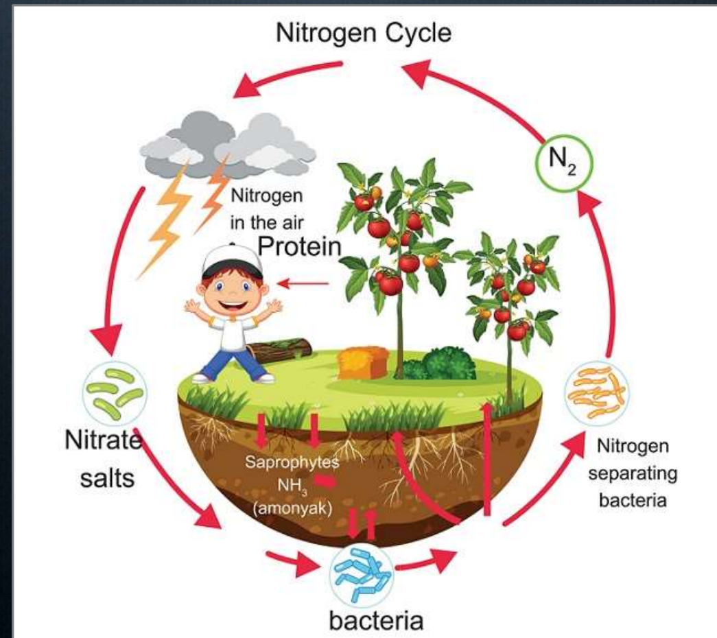
Nitrogen Cycle
