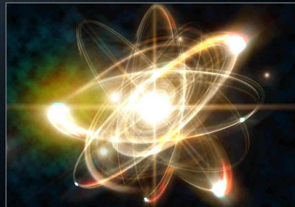
Electron Orbitals
