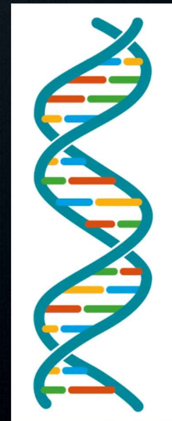
DNA
