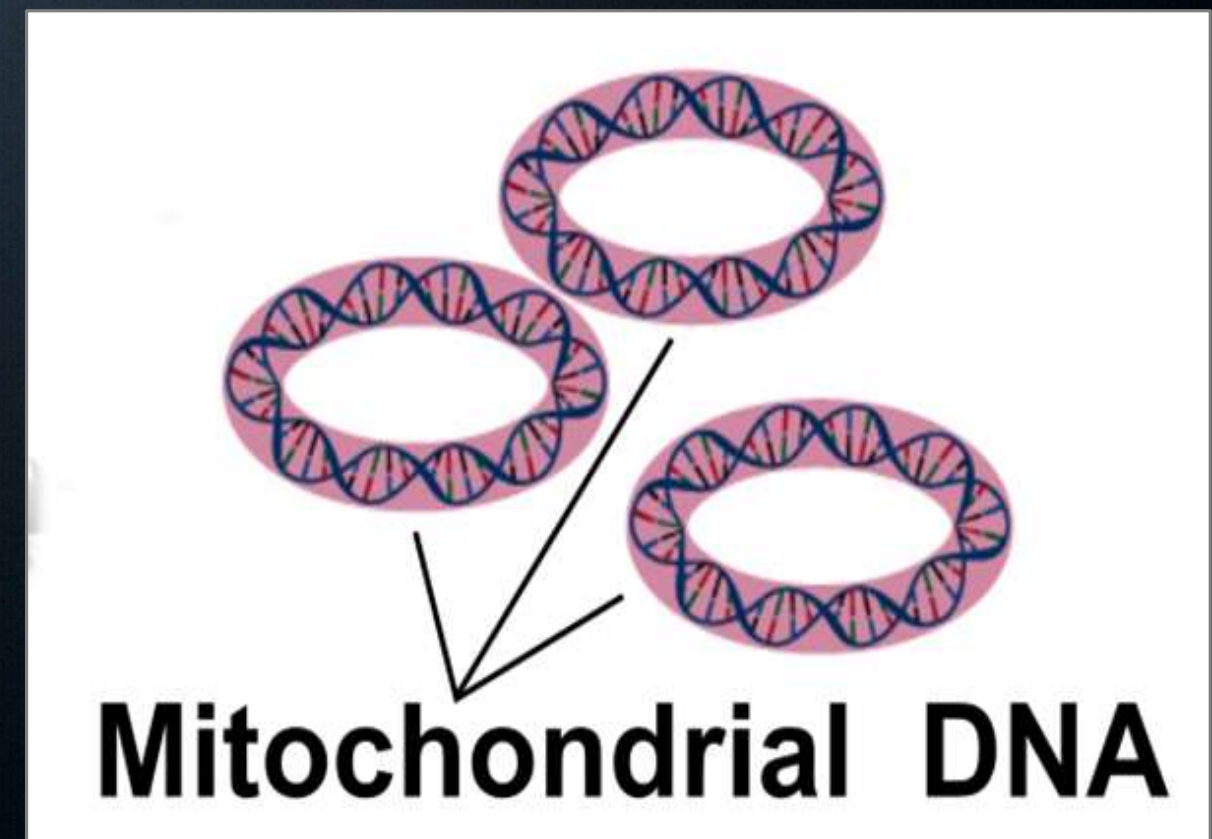
Mitochondrial DNA
